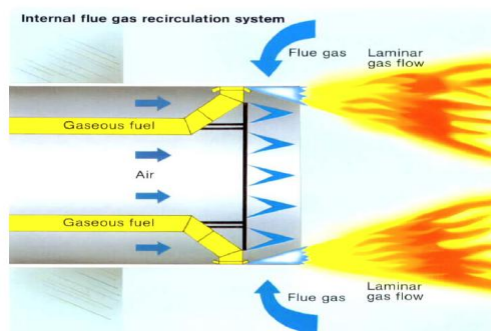
DELTA 燃烧火管—低氮氧燃
